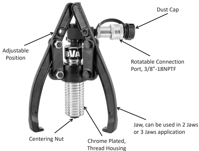
Figure 1: HGPT Series Major Components
