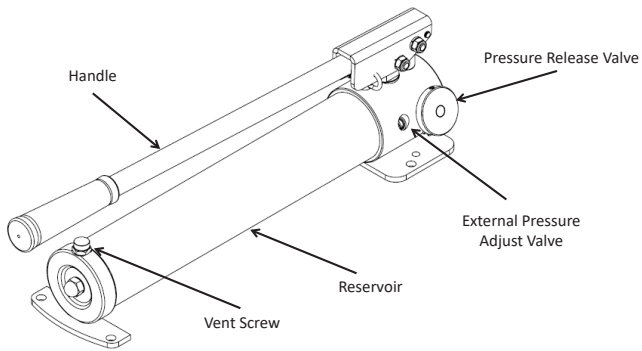
Figure 1 - P1000A Major Components
