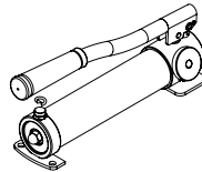
Figure 4 - Loosen vent screw counter-clockwise.
